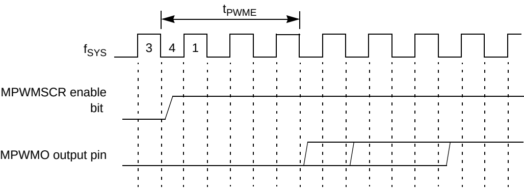
Figure F-48. MPWMSM Enable to MPWMO Output Pin Rising Edge Timing Diagram
