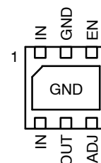
NCP691, NCP692 – 6 PIN DFN Adjustable Version (Bottom View)
