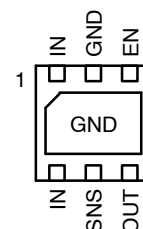
NCP691, NCP692 – 6 PIN DFN Fixed Version (Bottom View)
