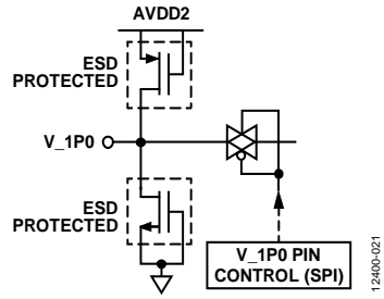
Figure 70. V_1P0 Input/Output
