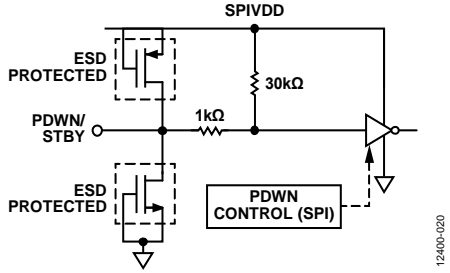
Figure 69. PDWN/STBY Input
