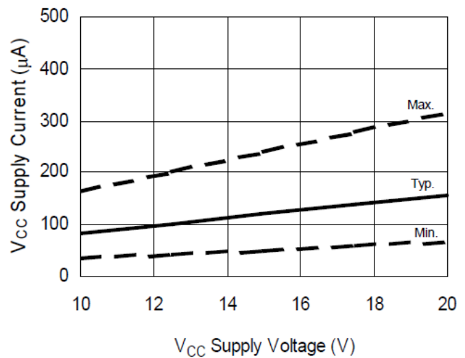
Figure 14B. V_{CC} Supply Current vs. Supply Voltage
