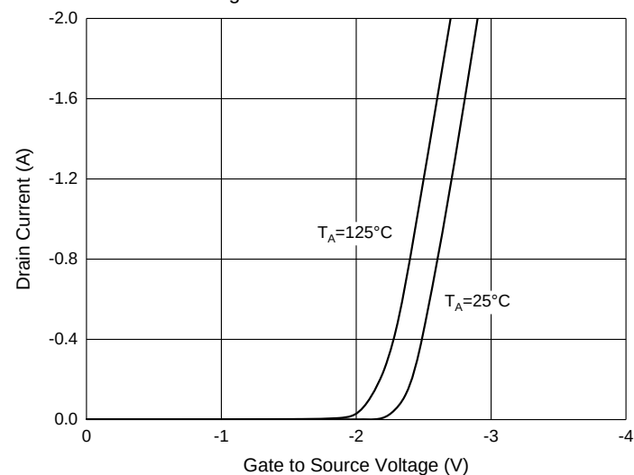
Fig. 3 - Transfer Characteristics
