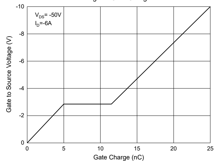
Fig. 4 - Gate Charge
