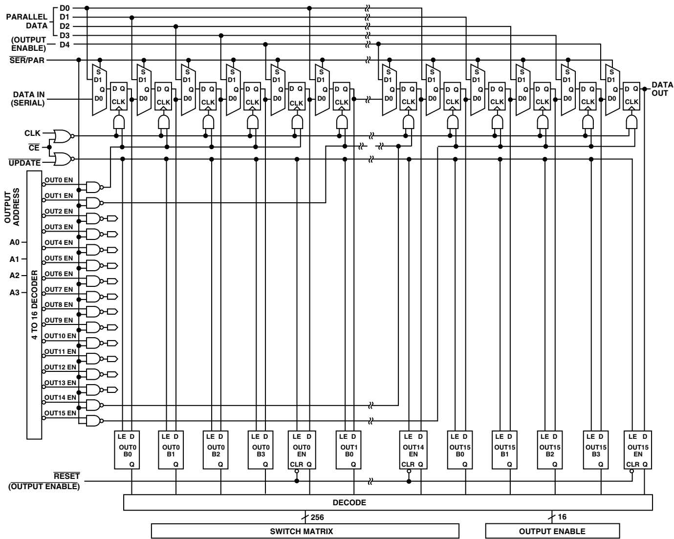
Figure 4. Logic Diagram
