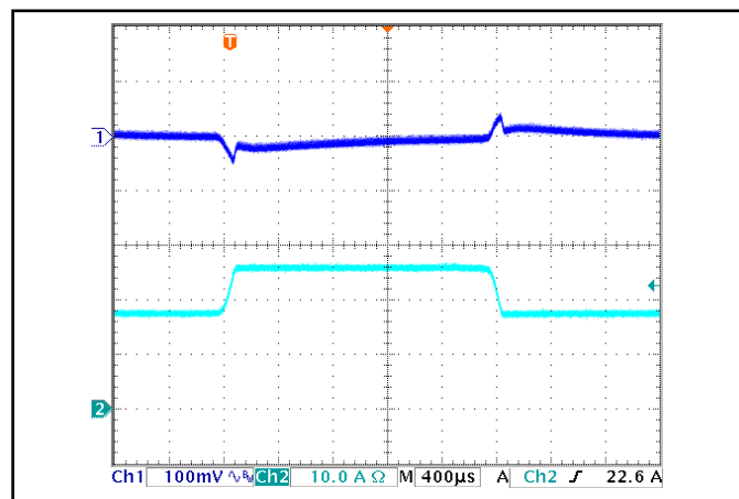
Figure 12: Output voltage response to step-change in load current (50%-75%-50% of I_{out(max)} ; dI/dt = 0.3 A/\mu s ). Load cap: 10μF, 100 mΩ ESR tantalum cap and 1μF ceramic cap. Ch 1: V_{out} (100mV/div), Ch 2: I_{out} (10A/div).
