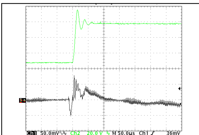
Figure 17: Output voltage response to step-change in input voltage (50V to 100V in 8\ \mu\text{s} ), at 17.5A load current. Load cap: 15\ \mu\text{F} 100\text{m}\Omega ESR tantalum capacitor and 1\ \mu\text{F} ceramic cap. Ch 1: V_{out} (50mV/div), Ch 2: V_{in} (20V/div).
