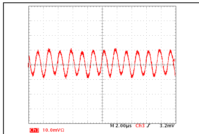
Figure 14: Input Terminal Ripple Current, i_c , at full rated output current and nominal input voltage with 10\ \mu\text{H} source impedance and 47\ \mu\text{F} electrolytic capacitor (100 mA/div). Bandwidth: 250MHz. See Figure 13.
