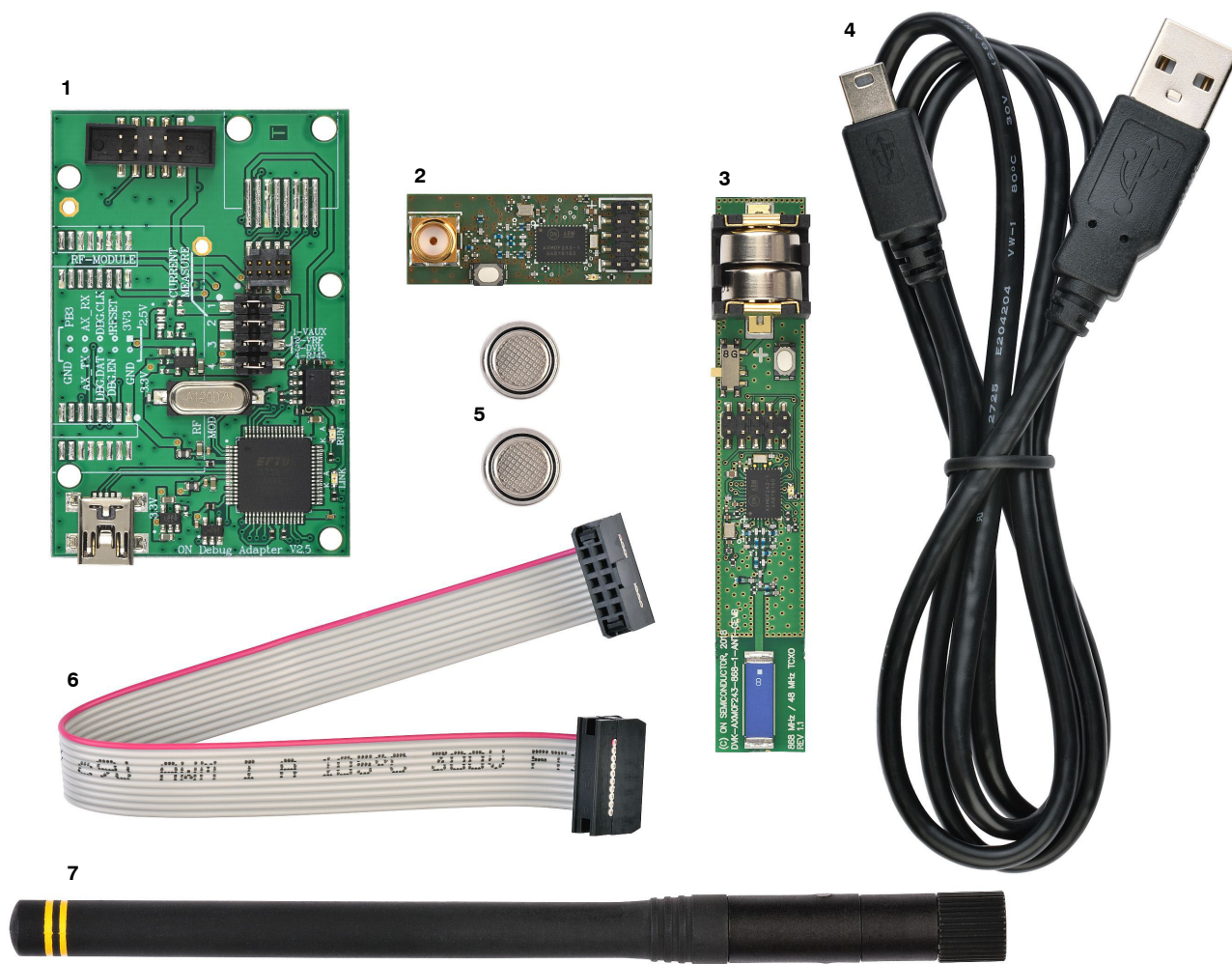
Figure 1. DVK-AXM0F243-868-x-GEVK Kit
