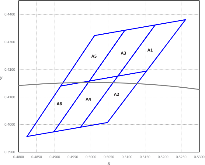
Figure 7. 3- and 5-step MacAdam ellipse illustration for Tables 6a-6i. Figure 8a. Color bin structure for LUXEON 3535L Line 2200K.
