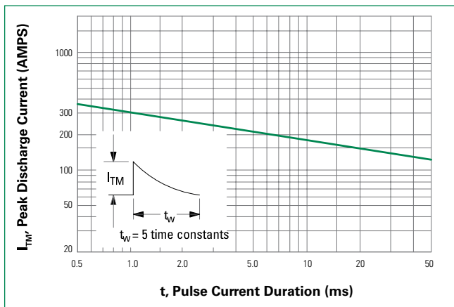
Figure 3. Current Derating
