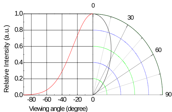
Radiation Characteristics
