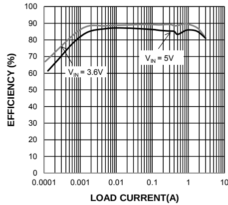
Efficiency vs. Load 1.8V_{OUT} @25°C
