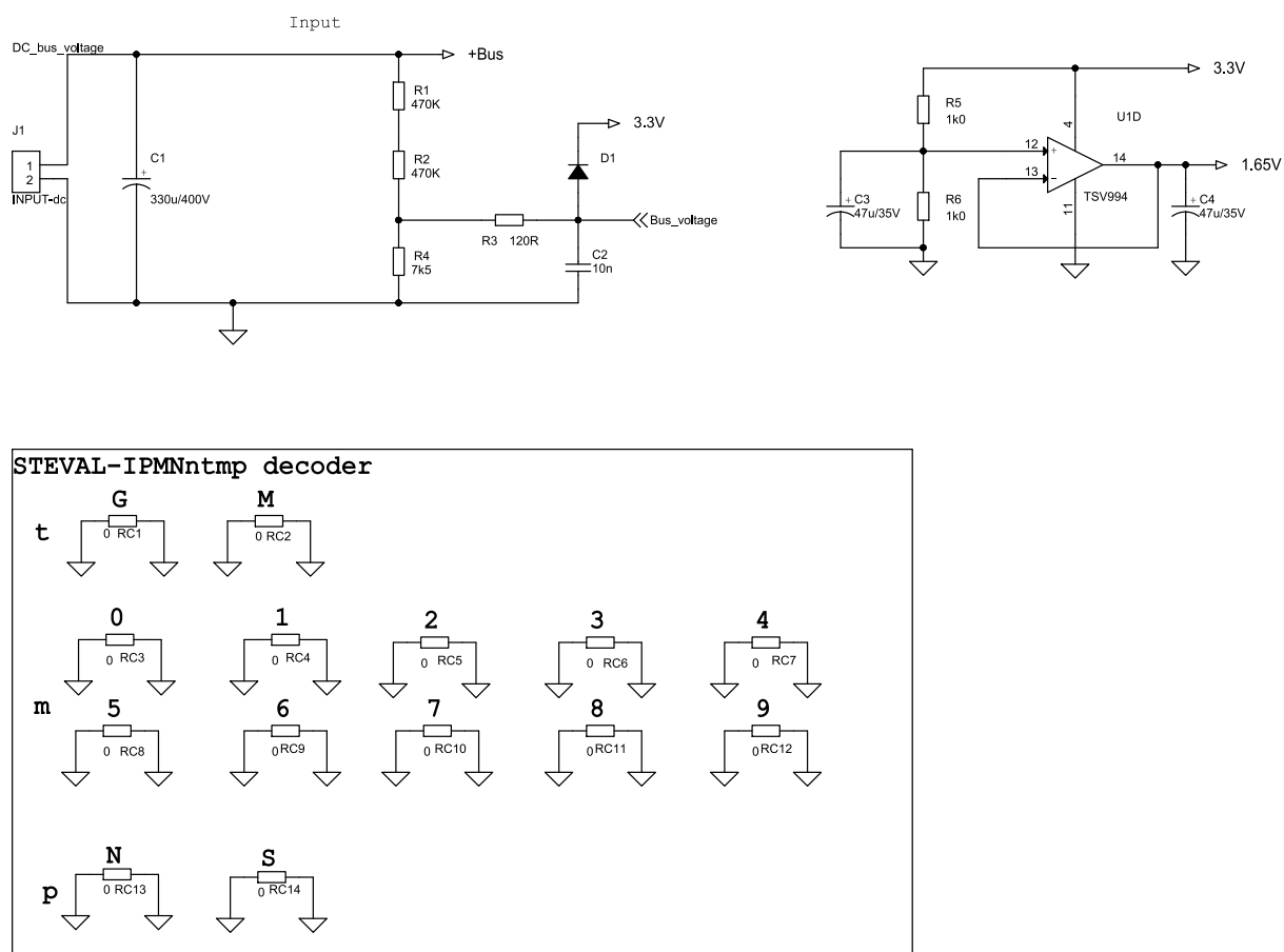
Figure 2. STEVAL-IPMnM1S - circuit schematic (1 of 5)
