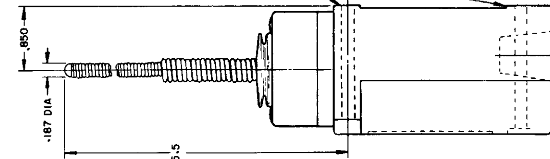
PLASTIC EXTENSION TYPE 7A ACTUATOR TYPE LSJ1 AND LSJ3
