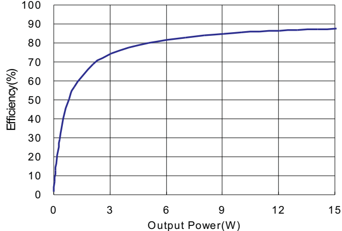
10. Efficiency vs Output Power ( V_{CC}=24V )
