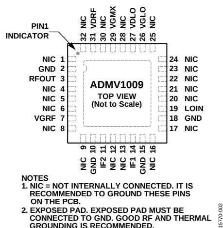
Figure 2. Pin Configuration
