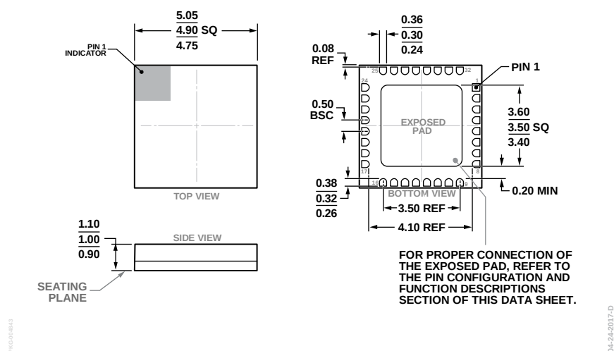
Figure 63. 32-Terminal Ceramic Leadless Chip Carrier [LCC] (E-32-1)
