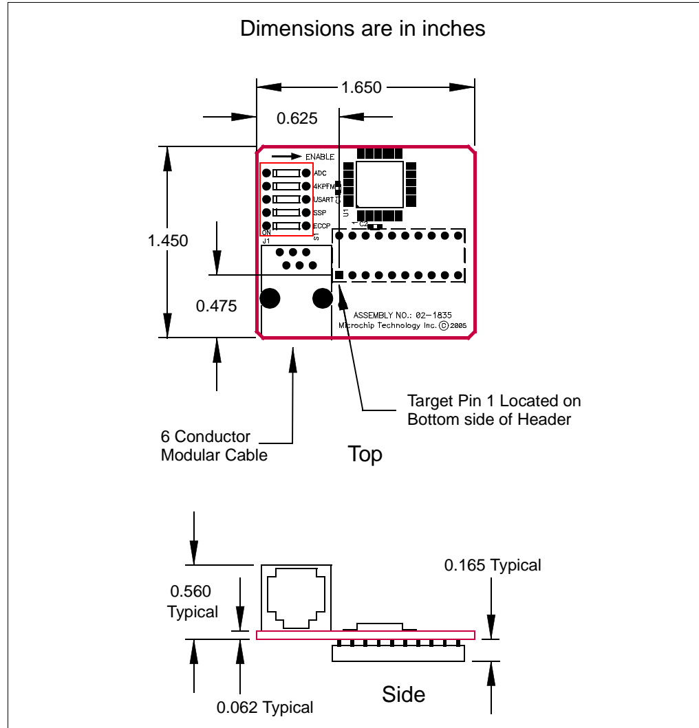
FIGURE 7: DIMENSIONS – AC162061
