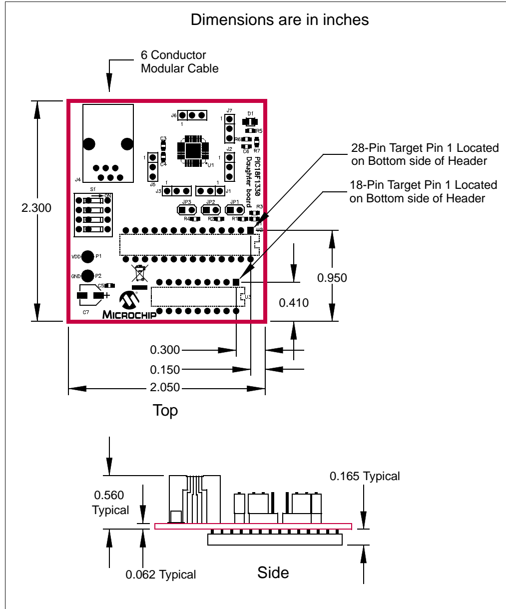
FIGURE 8: DIMENSIONS – AC162078
