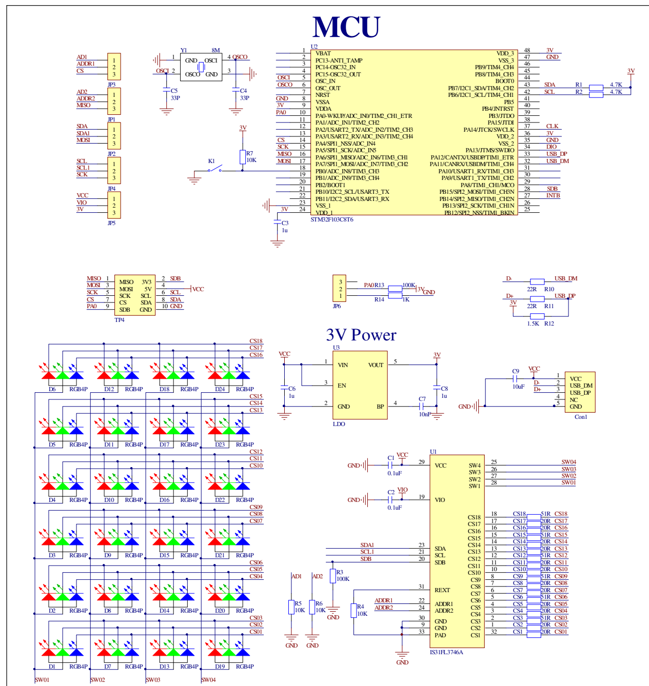
Figure 3: IS31FL3746A Application Schematic
