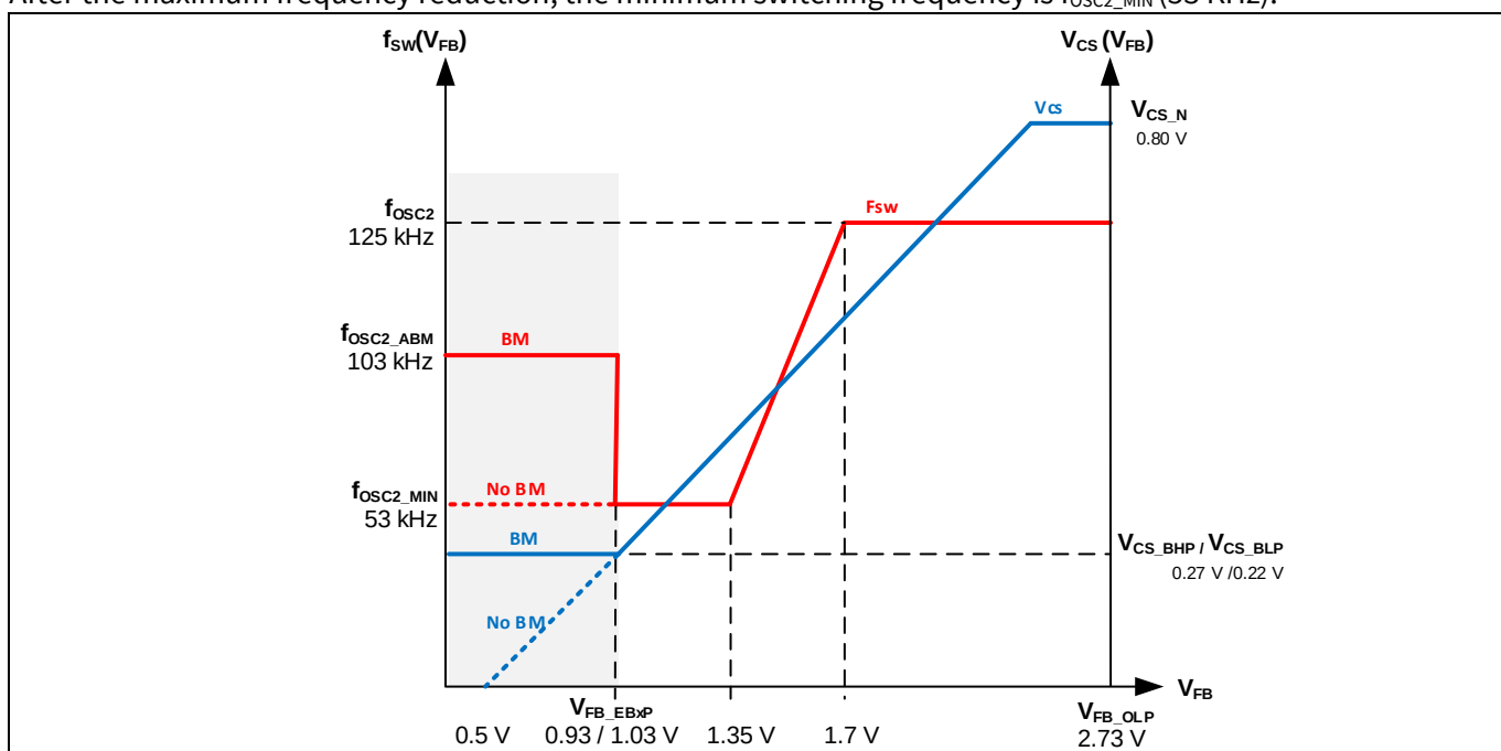
Figure 2 Frequency-reduction curve
