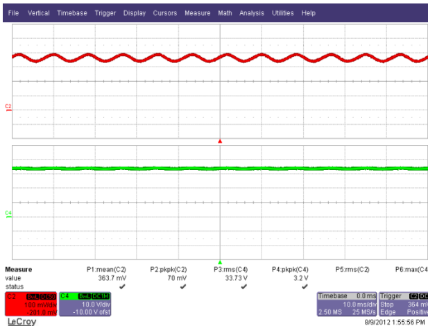
Figure 34 – 120 VAC, 60 Hz Full Load. Upper: I OUT , 100 mA / div. Lower: V OUT , 10 V, 10 ms / div.
