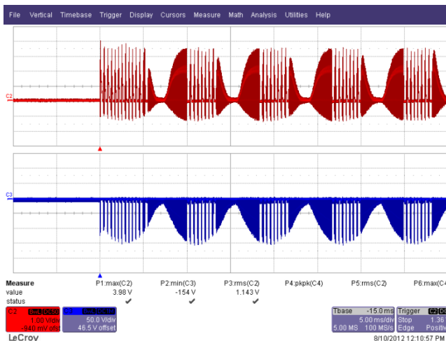
Figure 59 – 132 VAC, 60 Hz Output Short Condition. Upper: I_{D5} , 200 mA / div. Lower: V_{D5} , 50 V, 5 ms / div.
