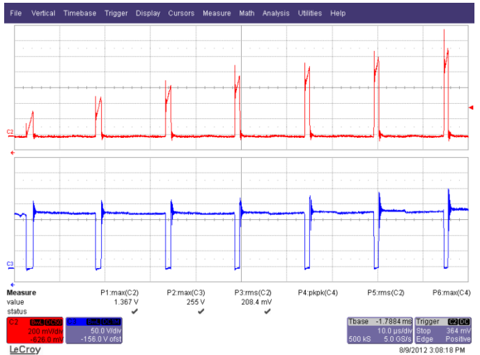
Figure 51 – 132 VAC, 60 Hz Start-up. Upper: I_{DRAIN} , 200 mA / div. Lower: V_{DRAIN} , 50 V, 10 \mu s / div.
