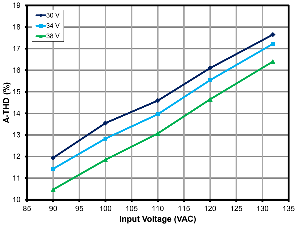
Figure 79 – A-THD vs. Line and Load.
