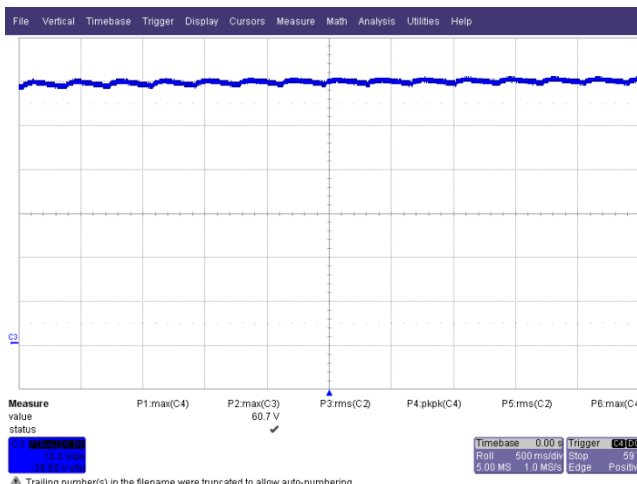
Figure 61 – 132 VAC, 60 Hz Open Load Condition. V_{OUT} , 10 V / div.
