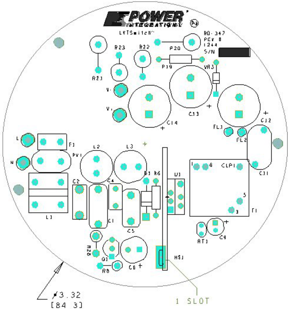
Figure 6 – Top Side.
