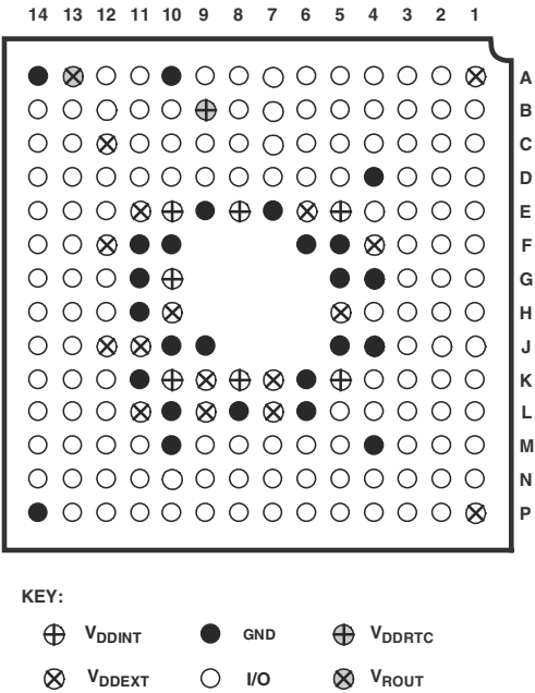
Figure 64. 182-Ball CSP_BGA Configuration (Bottom View)
