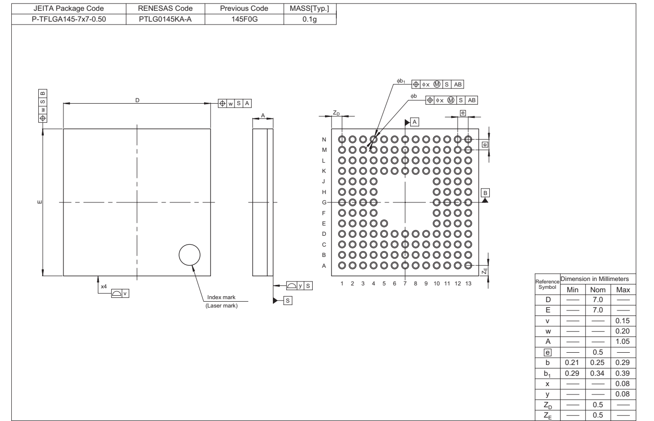
Figure 1.1 LGA 145-pin
