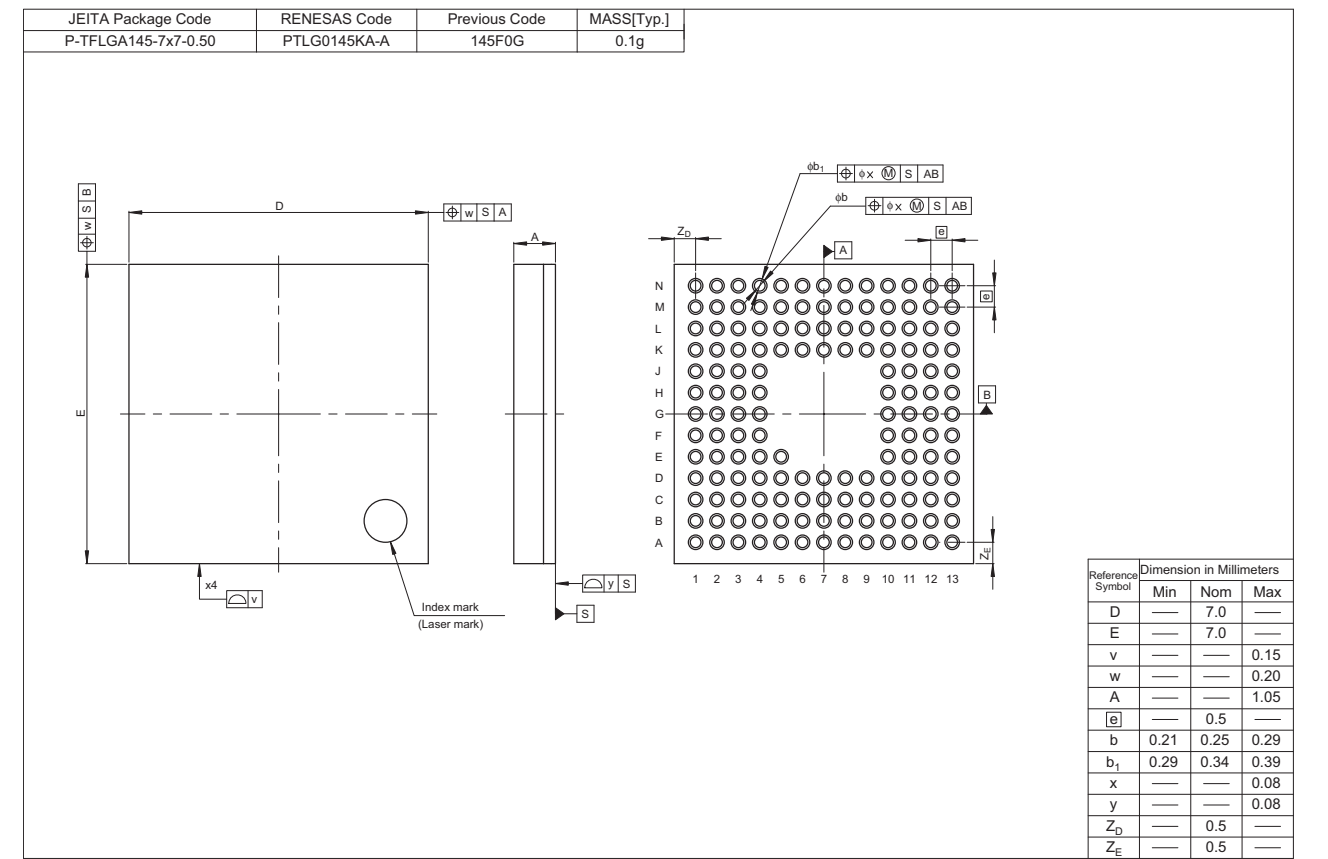
Figure 1.1 LGA 145-pin
