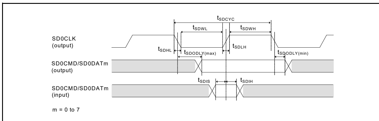
Figure 2.75 SD/MMC host interface signal timing
