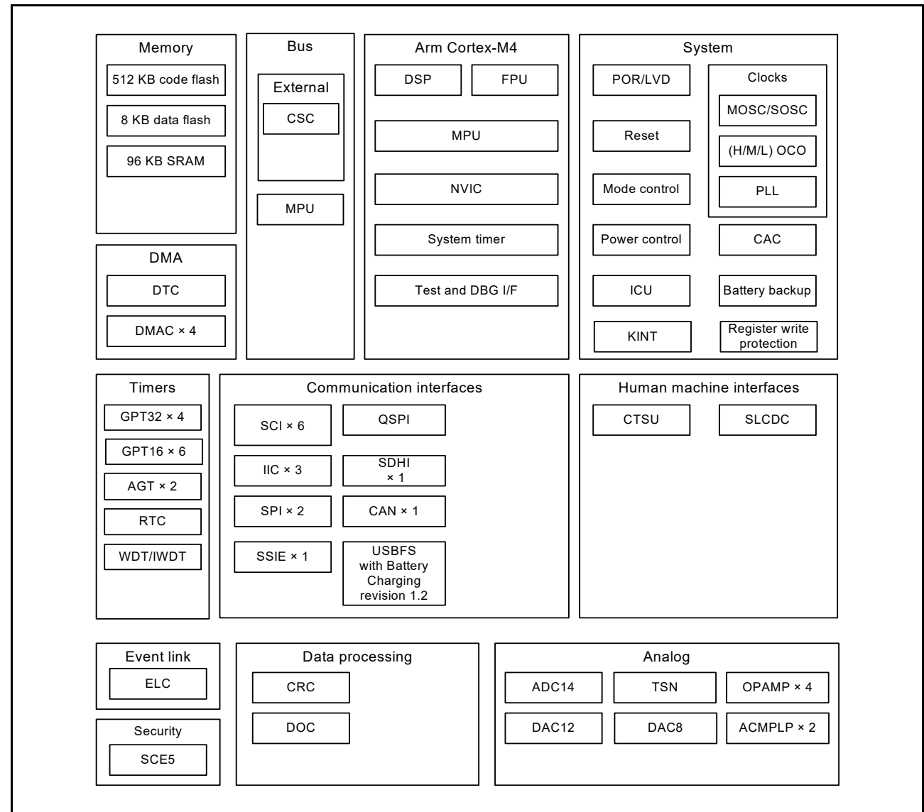
Figure 1.1 Block diagram
