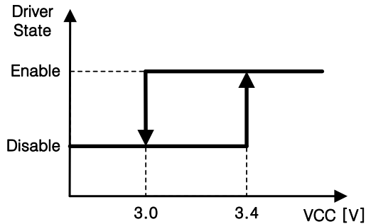
Figure 26. UVLO
