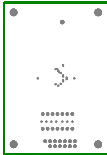
Figure 12. Layer 7, Ground
