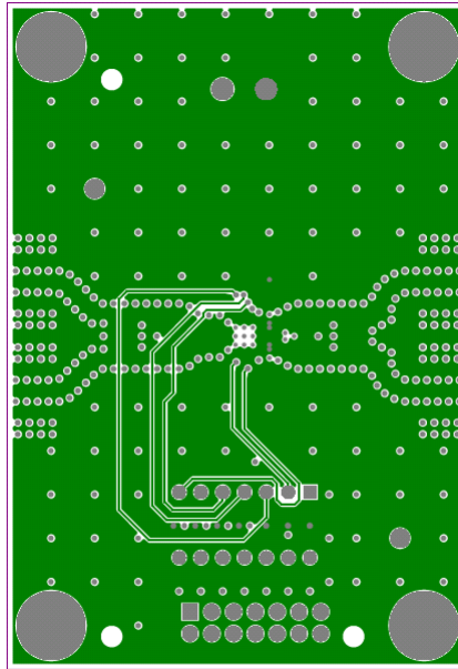
Figure 13. Layer 6, 5V Power
