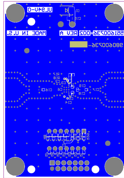
Figure 10. Bottom Layer
