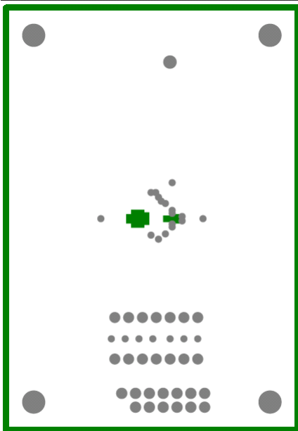
Figure 11. Layer 2, Ground
