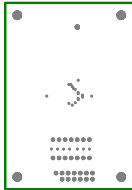
Figure 12. Layer 7, Ground
