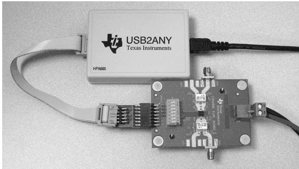
Figure 5. Evaluation Board
