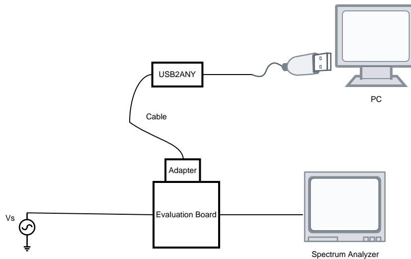
Figure 6. Typical Bench Setup
