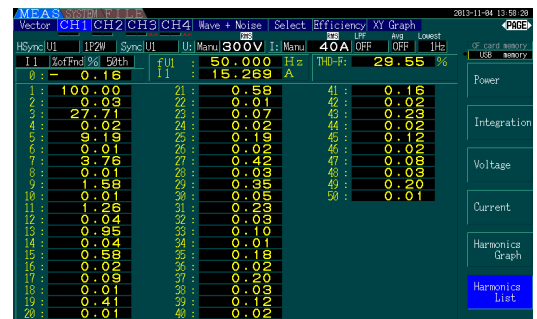
Figure 27. 75% Load
