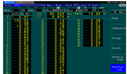
Figure 21. 25% Load
