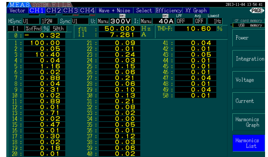
Figure 17. 25% Load
