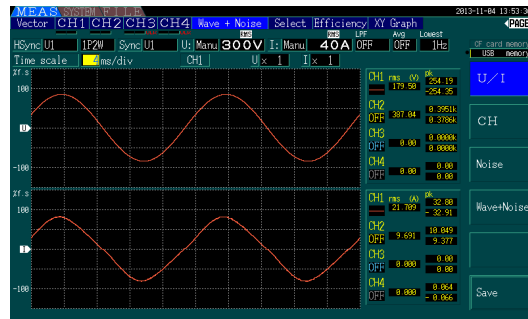
Figure 19. 75% Load
