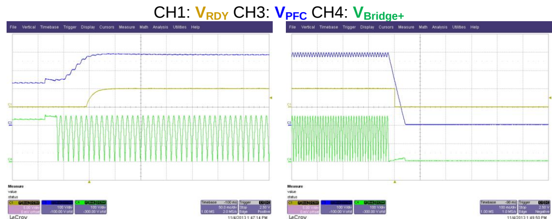
Figure 13. PFC ON
