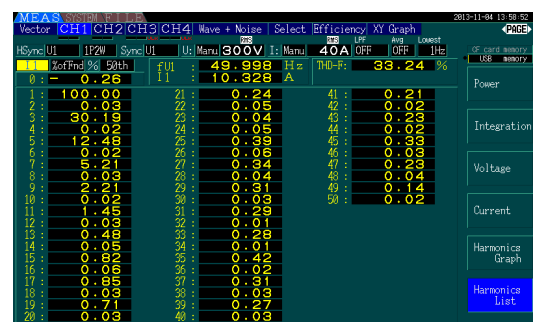
Figure 26. 50% Load
