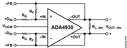
Figure 42. Circuit Definitions
