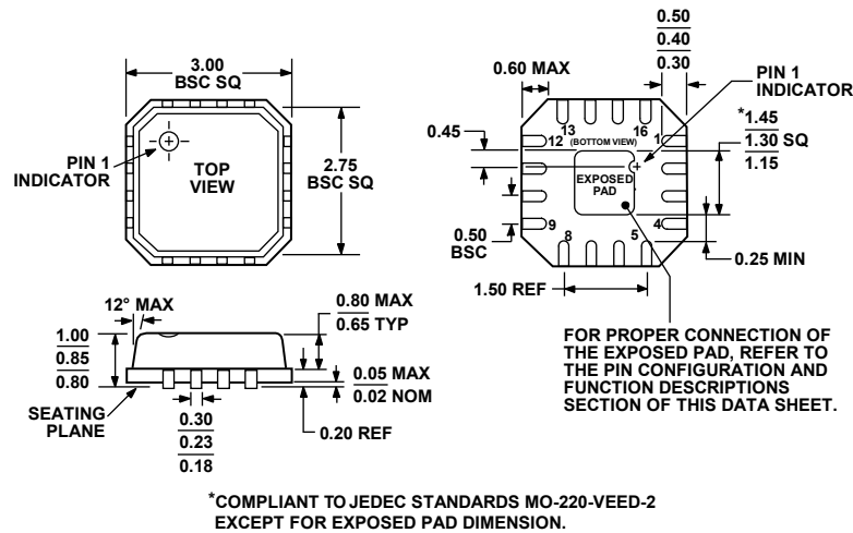
Figure 61. 16-Lead Lead Frame Chip Scale Package [LFCSP_VQ] 3 mm × 3 mm Body, Very Thin Quad (CP-16-2) Dimensions shown in millimeters
