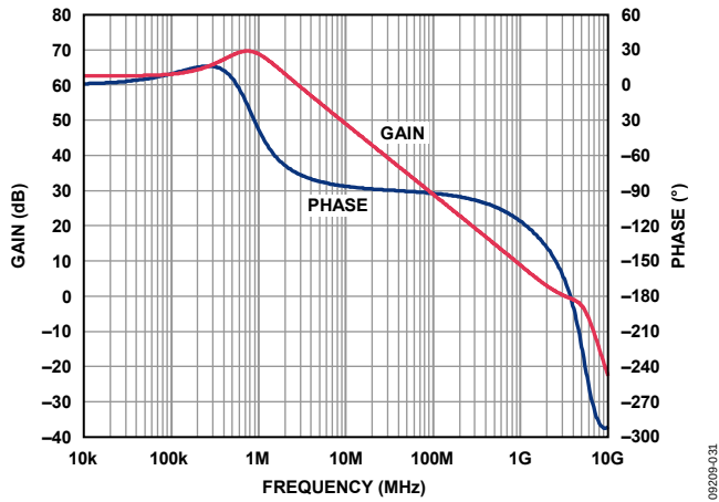
Figure 31. Open Loop Gain and Phase
