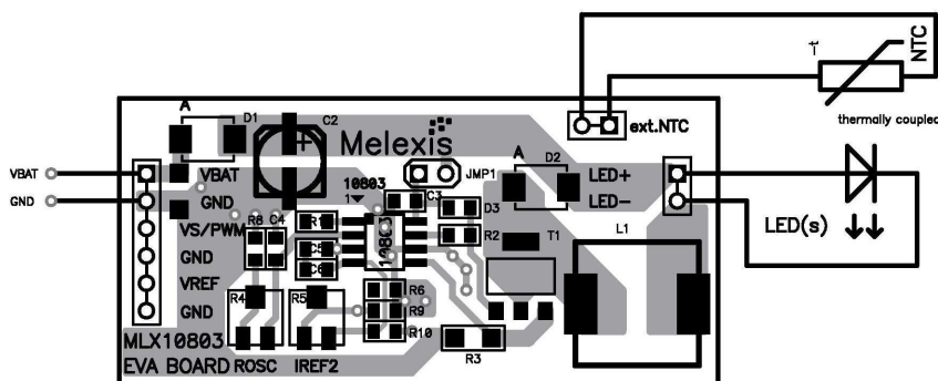
Figure 4: External NTC for temperature down regulation
