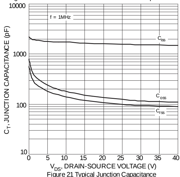
Figure 21 Typical Junction Capacitance
