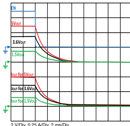
Figure 26 - Typical Fall Time C_{OUT} = 200 \mu F , C_{IN} = 4.7 \mu F , R_{OUT} = 10 \Omega
