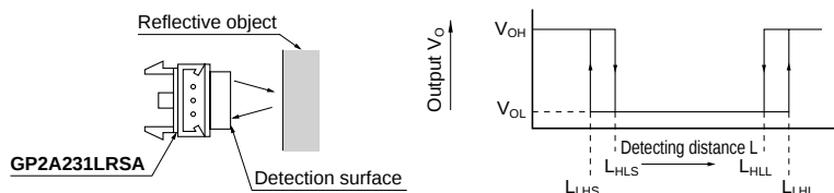
Fig.2 Test Condition for Detecting Distance Characteristics
