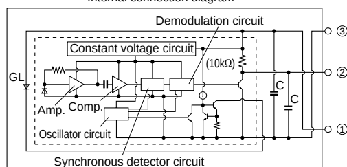
Internal connection diagram
