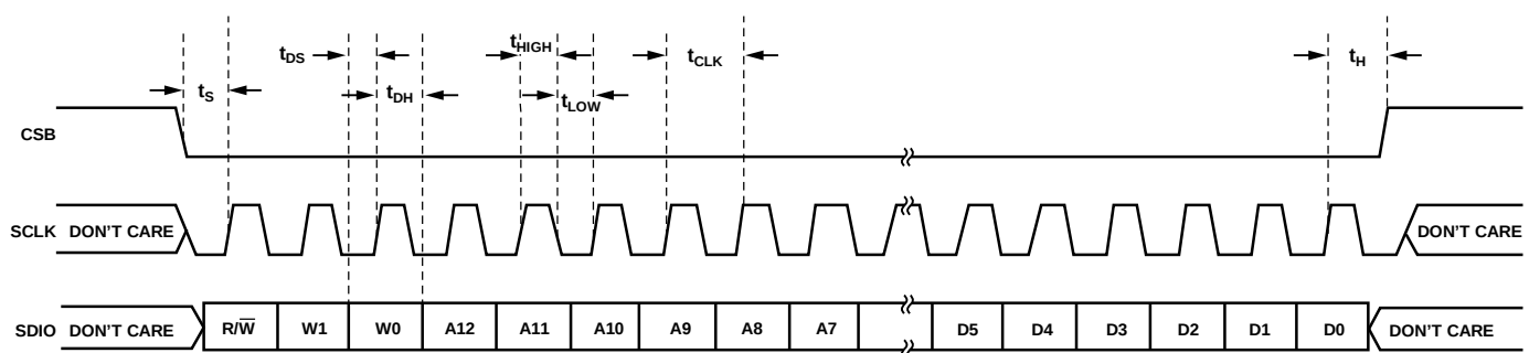
Figure 55. Serial Port Interface Timing Diagram
