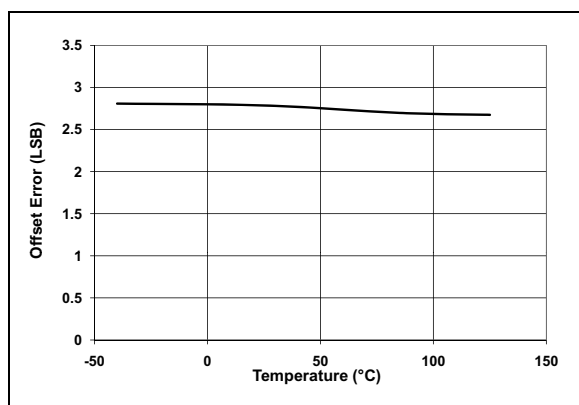
FIGURE 2-14: Offset Error vs. Temperature.
