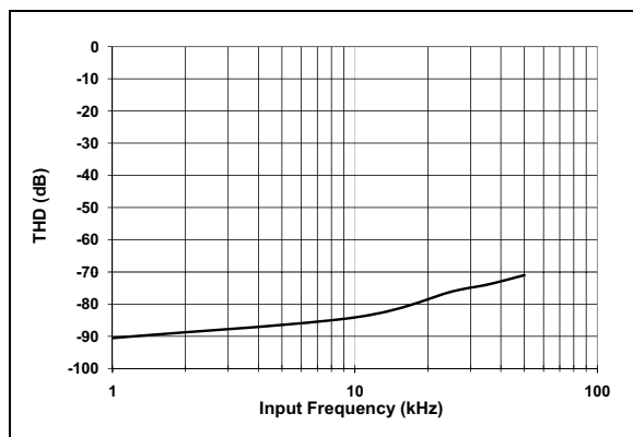
FIGURE 2-13: Total Harmonic Distortion (THD) vs. Input Frequency.
