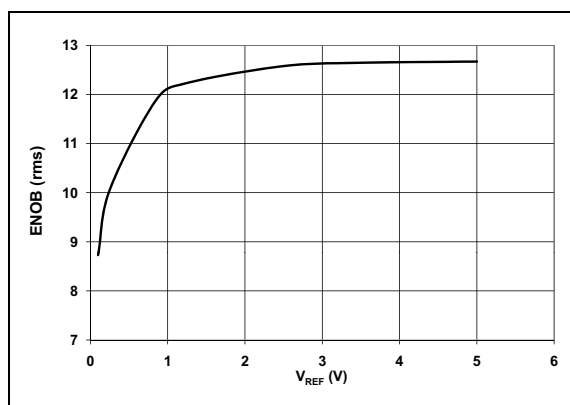
FIGURE 2-17: Effective Number of Bits (ENOB) vs. V_{REF} .
