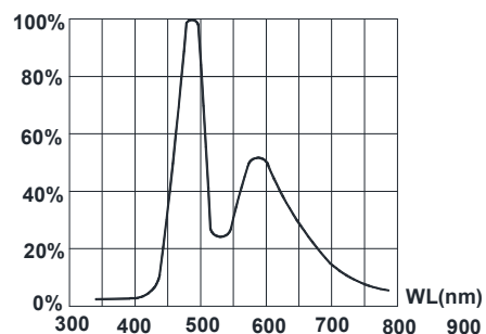
FIG.4 RELATIVE LUMINOUS INTENSITY VS. WAVELENGTH. 50% Power Angle : 120°
