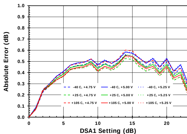
Figure 21. DSA1 Absolute Attenuation Error (INL)
