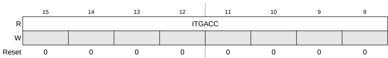
Figure 21-8. Integration Accumulator Register High (ITGACC)
