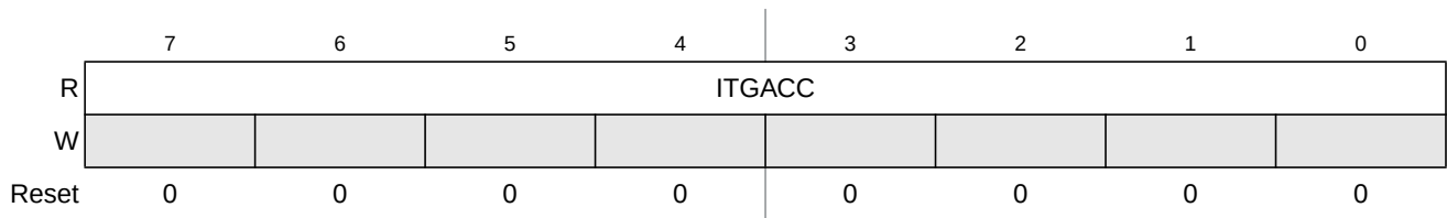
Figure 21-9. Integration Accumulator Register Low (ITGACC)
