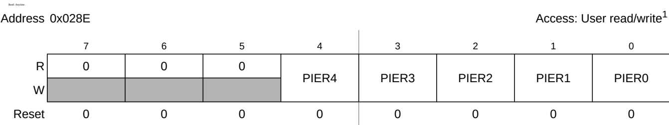
Figure 2-76. Port R Interrupt Enable Register (PIER)
