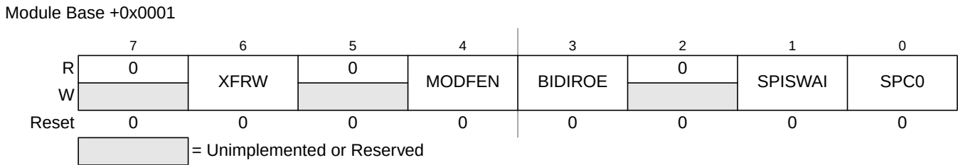
Figure 15-4. SPI Control Register 2 (SPICR2)
