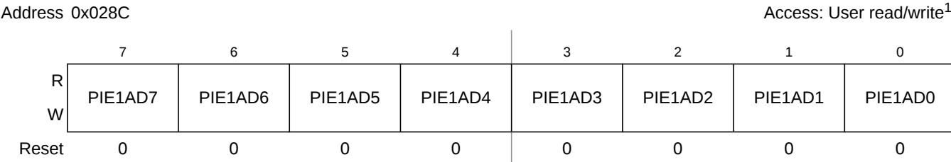
Figure 2-74. Port AD Interrupt Enable Register (PIE1AD)
