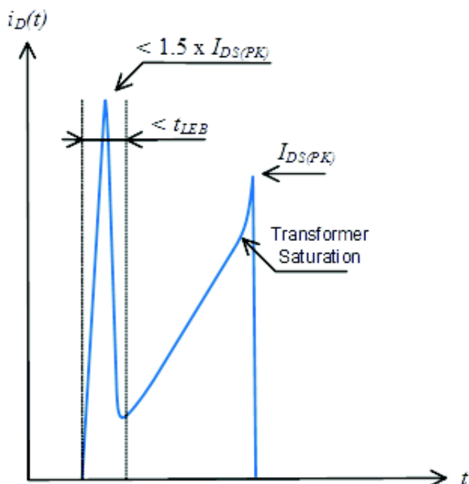
Figure 4. Spike Limits
