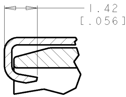
SECTION Z-Z SCALE 10:1
