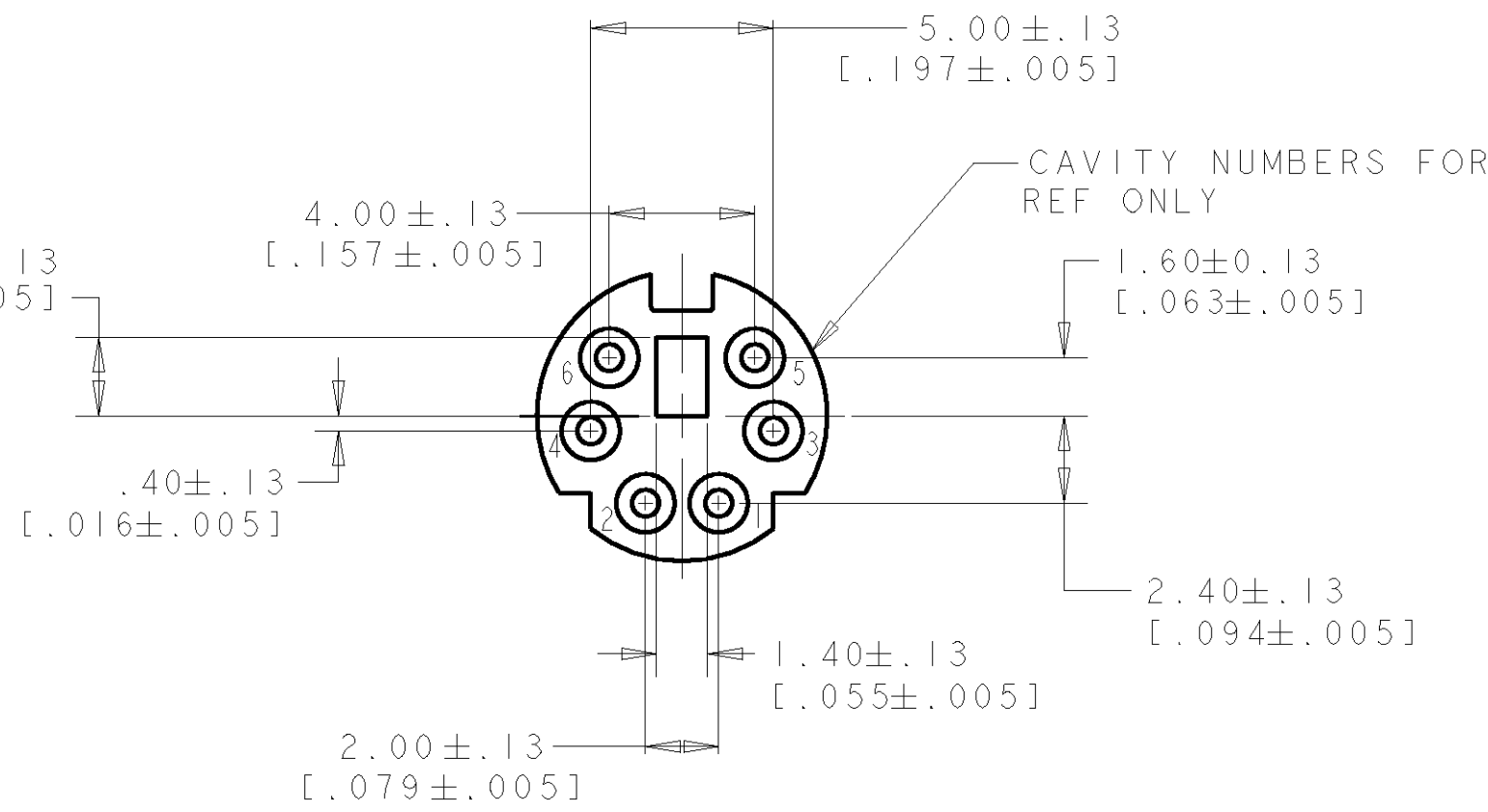
DETAIL D 6 PIN FACE
