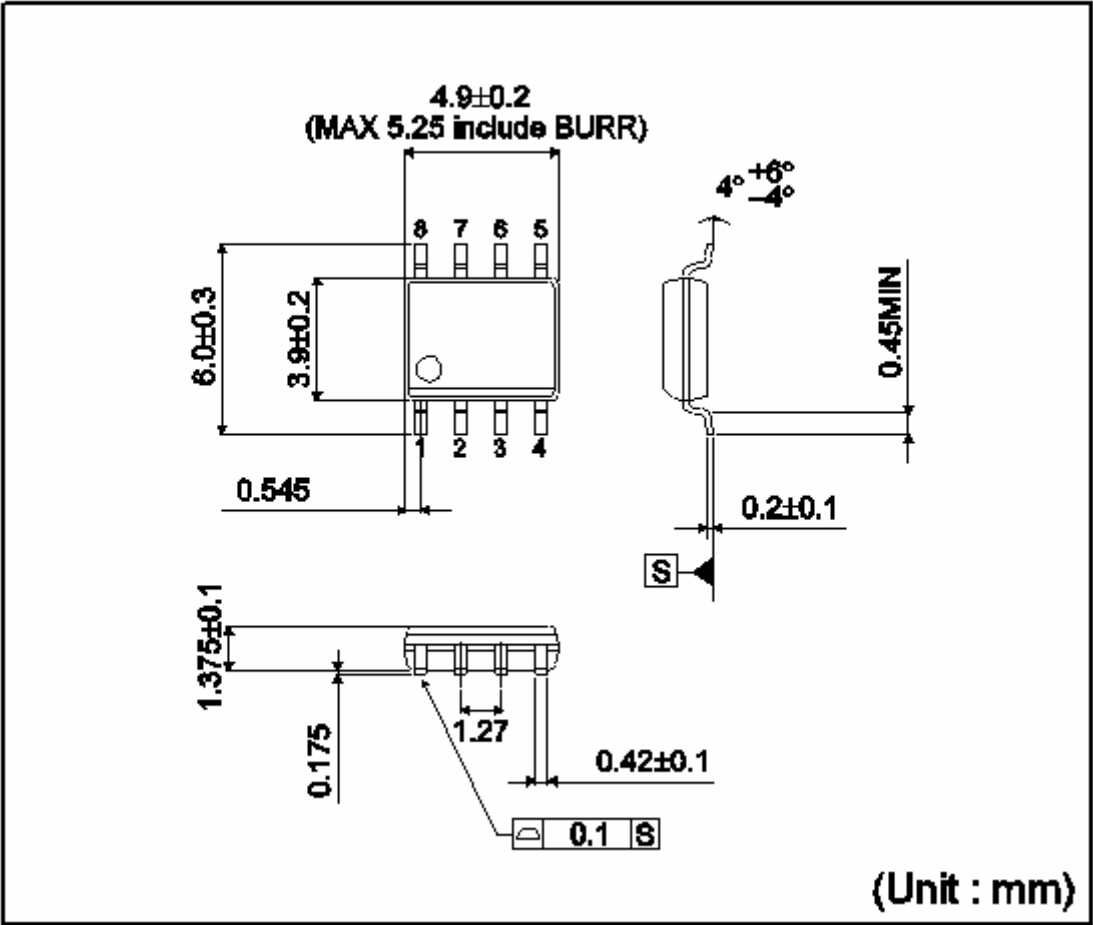
SOP-J8
