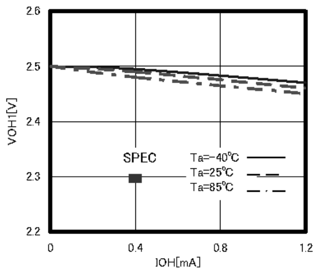
Figure 7. "H" Output Voltage V_{OH1} ( V_{CC}=2.5V )
