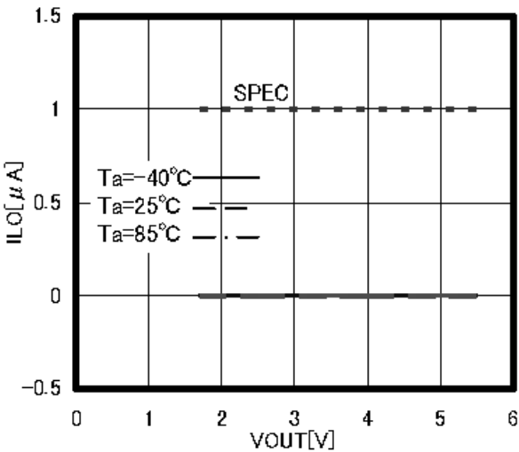
Figure 9. Output Leak Current I LO (SO)
