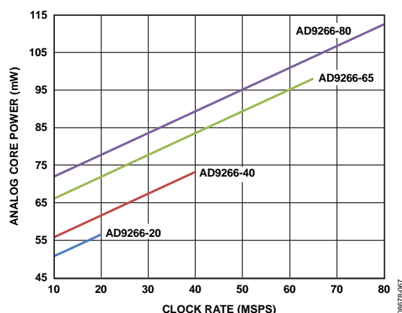
Figure 53. Analog Core Power vs. Clock Rate
