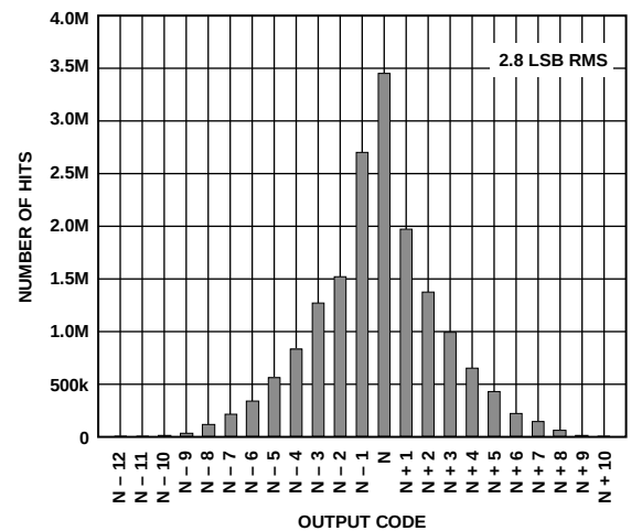
Figure 15. Grounded Input Histogram
