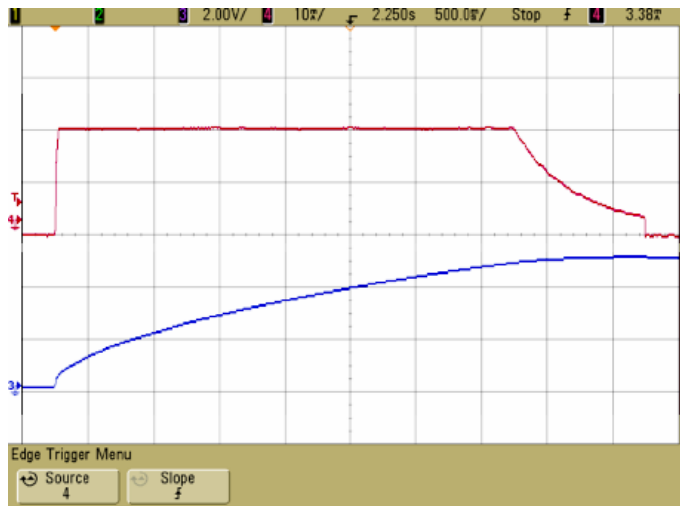
Figure 4. Charging Mode, V_{SYS} 2.5V, Input Current Set to 2.0, Ch 4 (Red) Input Current, 1.0A/DIV, Ch3 (Blue) VCAP Voltage
