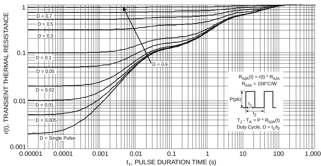
Fig. 14 Transient Thermal Response
